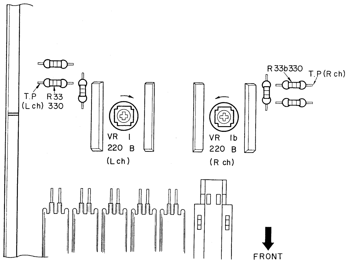
Fig. 4 Adjustment Points
