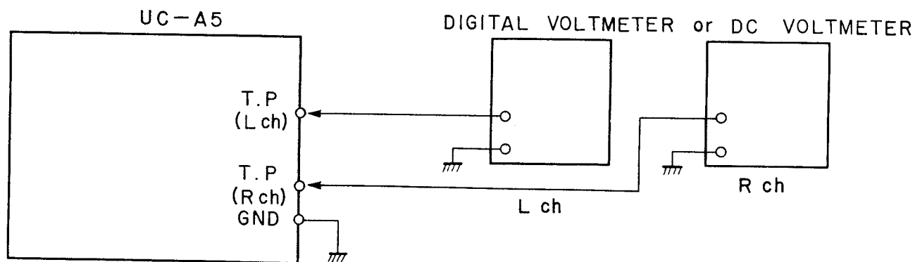
Fig. 5 Instrument Connections
