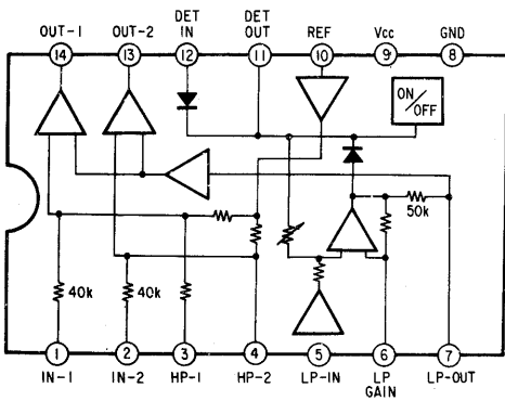
IC303 CXA-1249M
