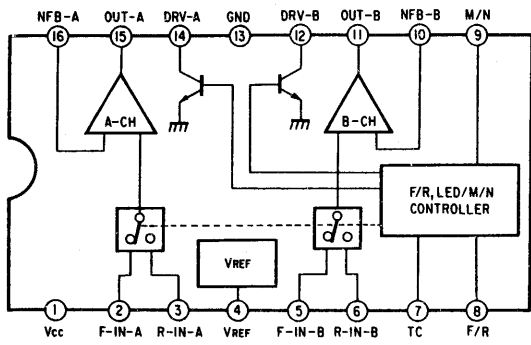
IC301 TA7795F
